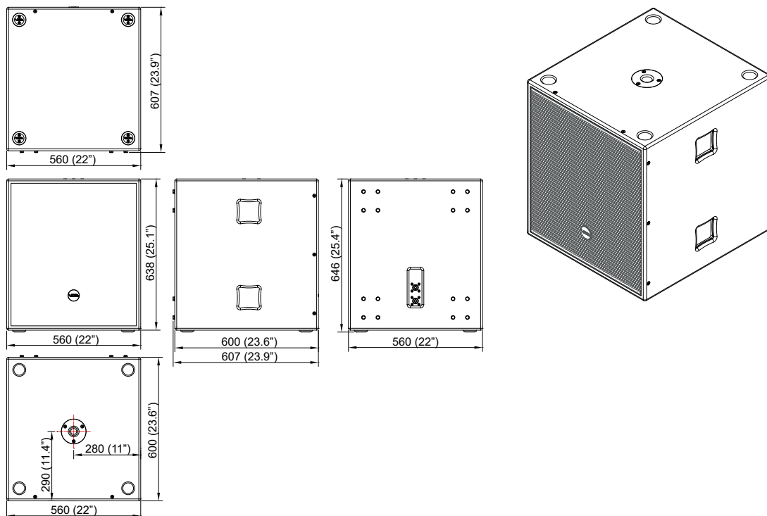
Figure 4.1: Dimensions
