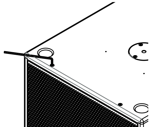
Figure 7.4: Bolt removal
