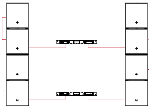
Figure 5.9: 8 x Stasys 118: 4 \Omega per channel / 2 amplifier
