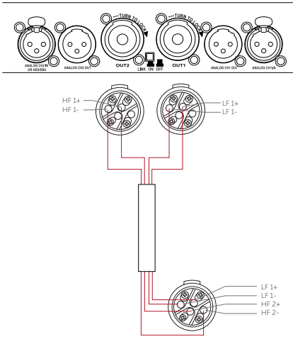
Figure 5.10: Bias V3 active mode
