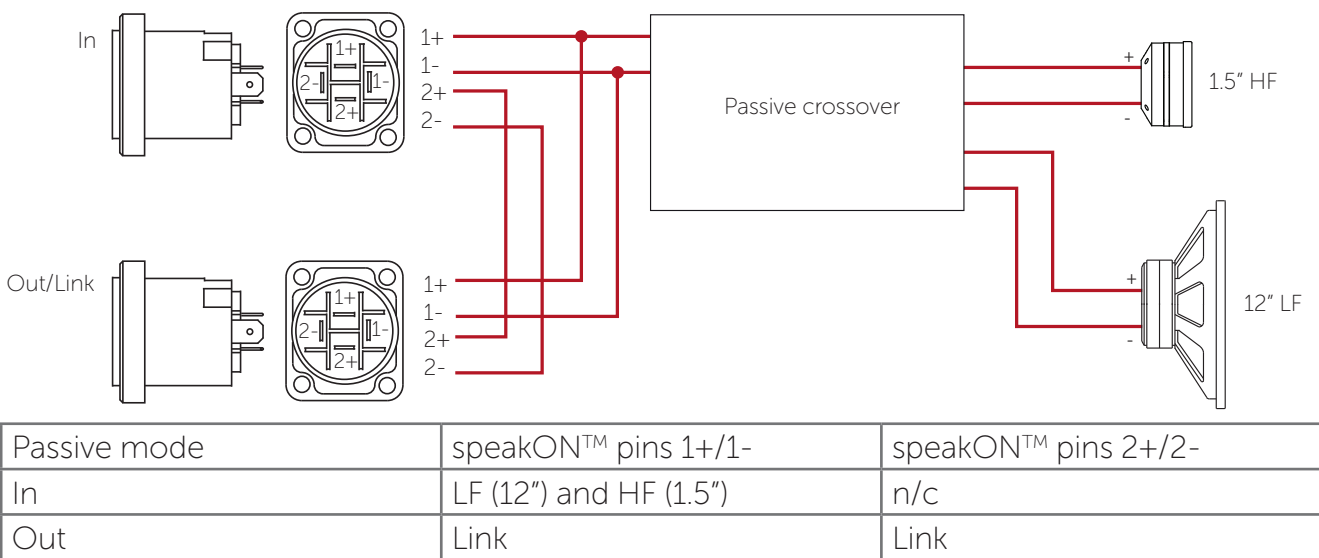
Figure 5.2: Stasys 2 passive mode wiring diagram
