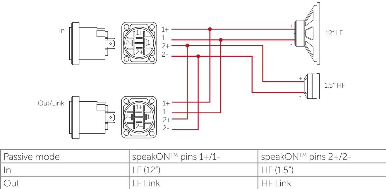
Figure 5.3: Stasys 2 active mode wiring diagram
