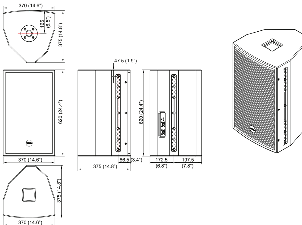
Figure 4.1: Dimensions
