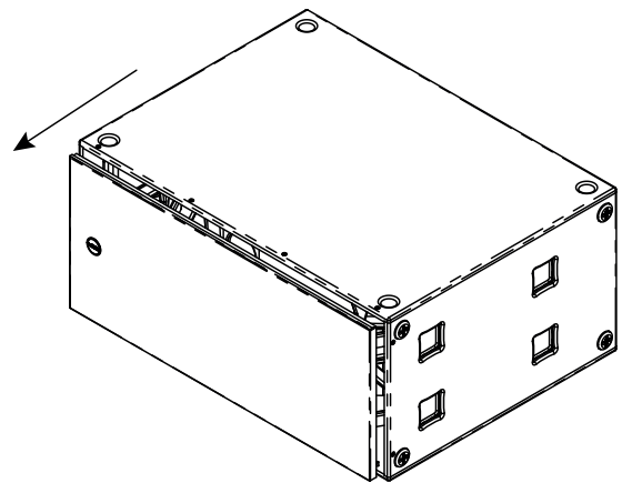
Figure 7.5: Grille removal
