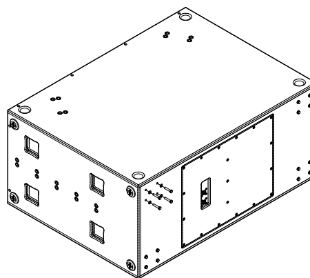
Figure 7.3: Bolt tightening
