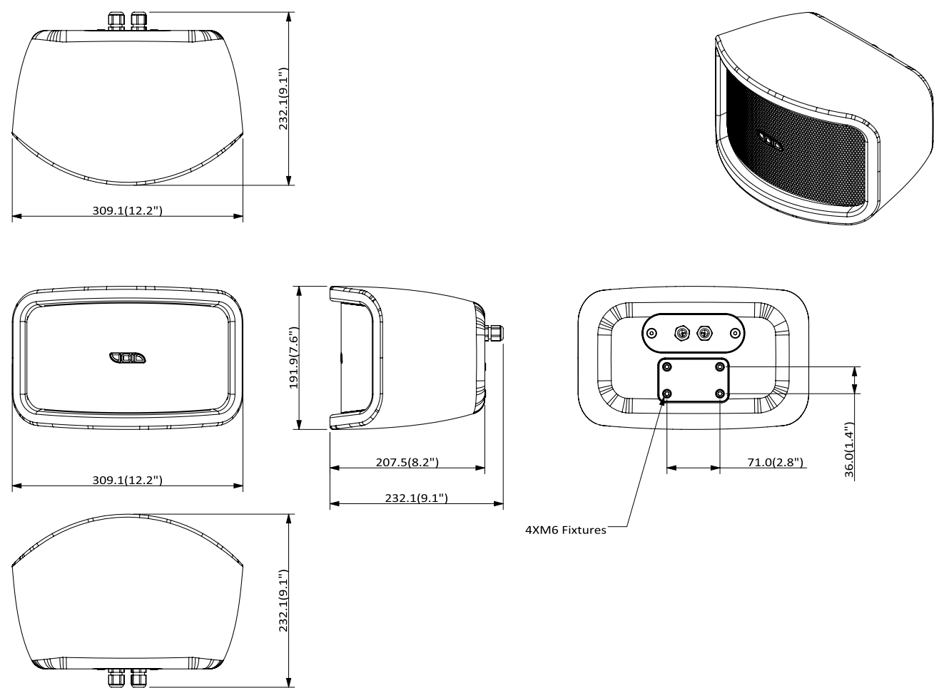
Figure 3.3: Dimensions
