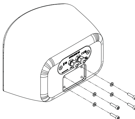
Figure 5.16: Bolt removal
