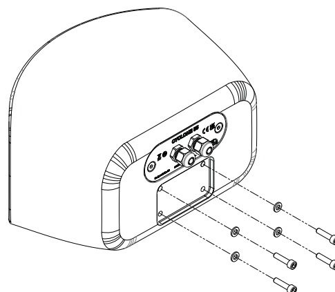
Figure 5.2: Bolt removal
